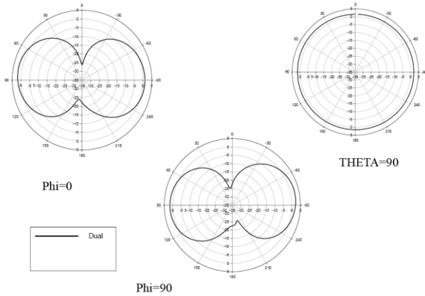
2D PATTERN_2.4GHZ
